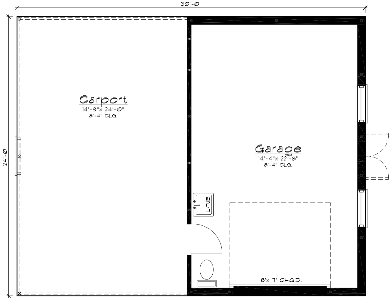
0 2' 4' 1 A2 FLOOR PLAN
