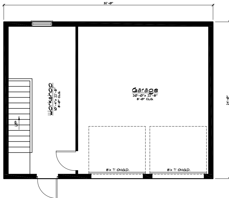
0 2' 4' 1 FLOOR PLAN (1st. Sty.) B2
